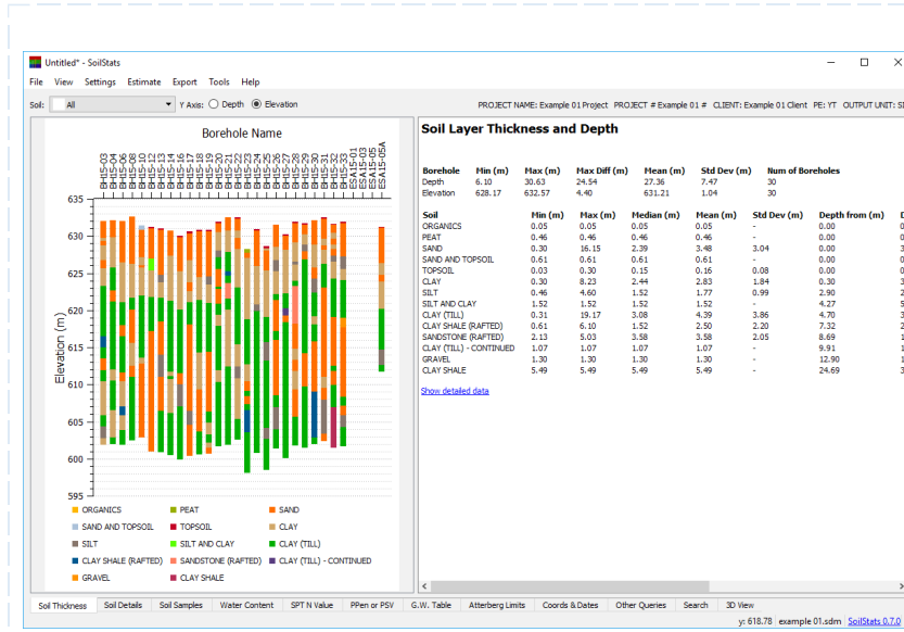
Summarize soil layer depths and thicknesses by soil layers
