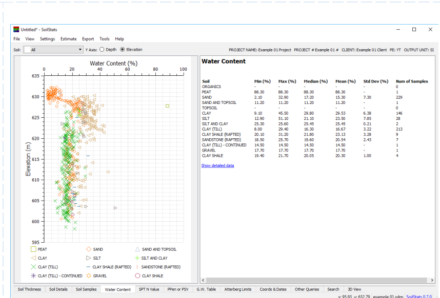
Summarize soil natural water contents by soil layers
