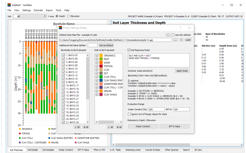
Regroup soil layers and assign soil layer colors
