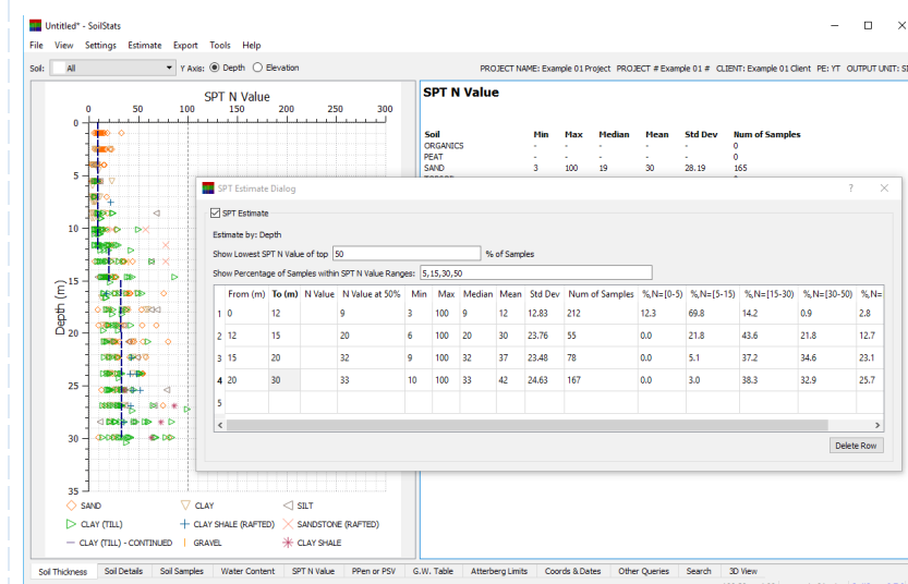
Estimate SPT "N" values by depth or elevation
