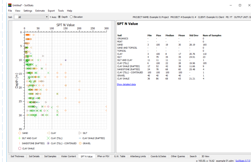
Summarize SPT "N" values by soil layers
